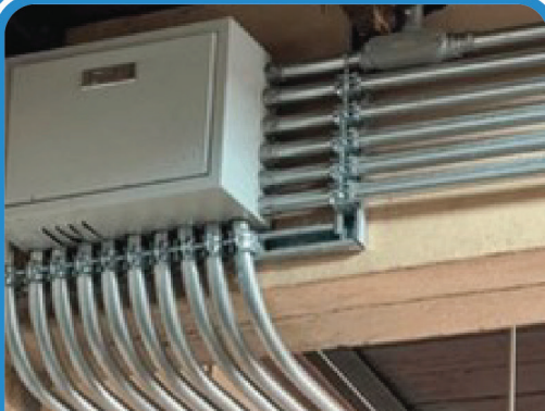
ELECTRICAL EMT CONDUITING WORK
